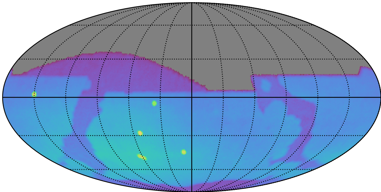
roll_uniform_eh_acc1.0_mjdp0_v3.4_10yrs : Brown Dwarf, L4
