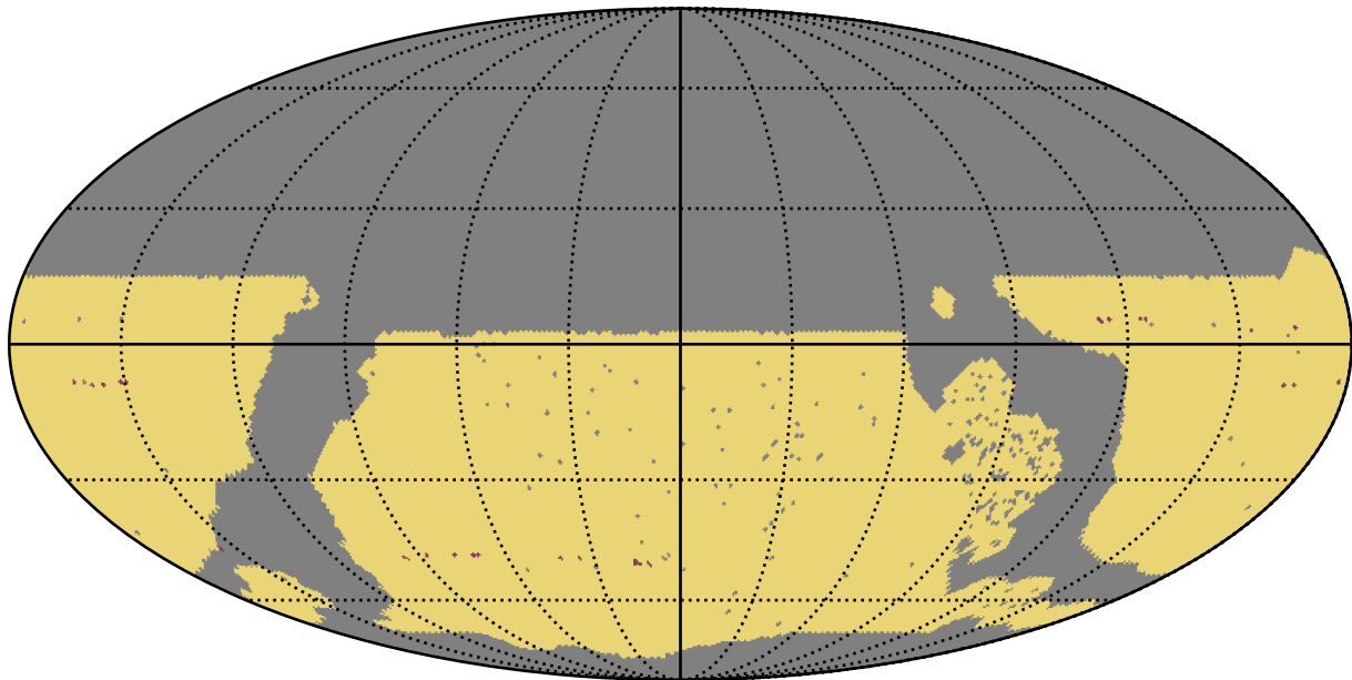
roll_uniform_eh_acc1.0_mjdp0_v3.4_10yrs WFD: RapidRevisits
