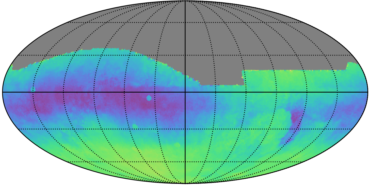
roll_uniform_eh_acc1.0_mjdp0_v3.4_10yrs All sky: Parallax-DCR degeneracy @ 24.0
