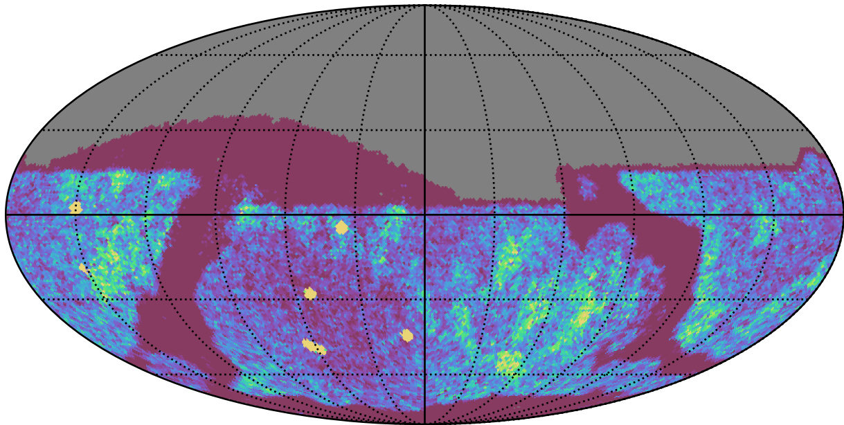
roll_uniform_eh_acc1.0_mjdp0_v3.4_10yrs Yr 1 z band: NVisits
