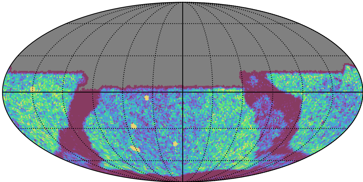
roll_uniform_eh_acc1.0_mjdp0_v3.4_10yrs Yr 1 y band: NVisits
