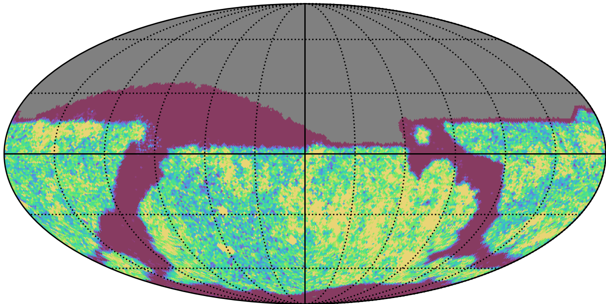
roll_uniform_eh_acc1.0_mjdp0_v3.4_10yrs Yr 1 i band: NVisits
