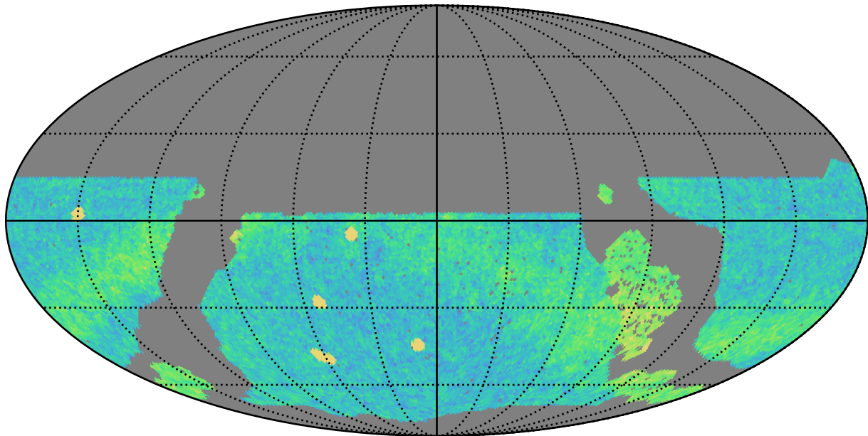
roll_uniform_eh_acc1.0_mjdp0_v3.4_10yrs WFD r band: NVisits
