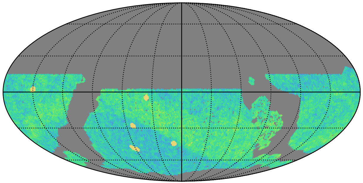
roll_uniform_eh_acc1.0_mjdp0_v3.4_10yrs WFD i band: NVisits
