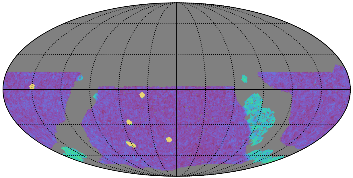
roll_uniform_eh_acc1.0_mjdp0_v3.4_10yrs WFD g band: NVisits
