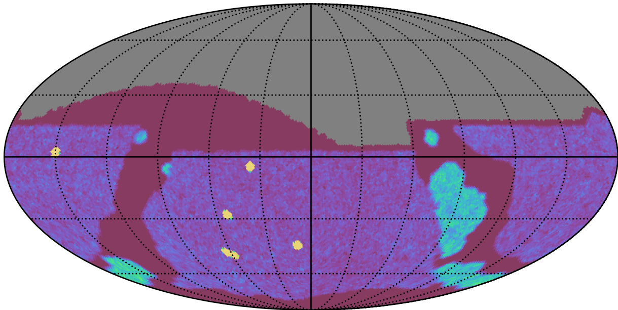
roll_uniform_eh_acc1.0_mjdp0_v3.4_10yrs All sky g band: NVisits
