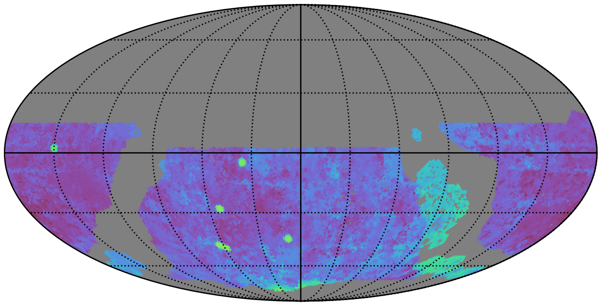
roll_uniform_eh_acc1.0_mjdp0_v3.4_10yrs WFD g band: Median Season Length
