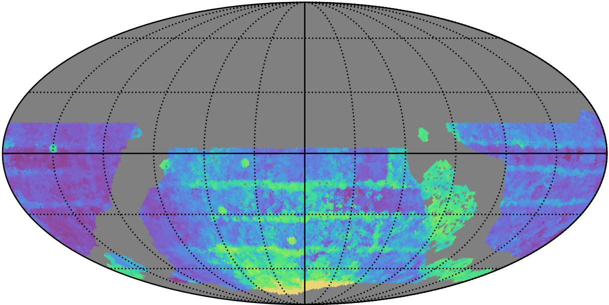
roll_uniform_eh_acc1.0_mjdp0_v3.4_10yrs WFD all bands: Median Season Length
