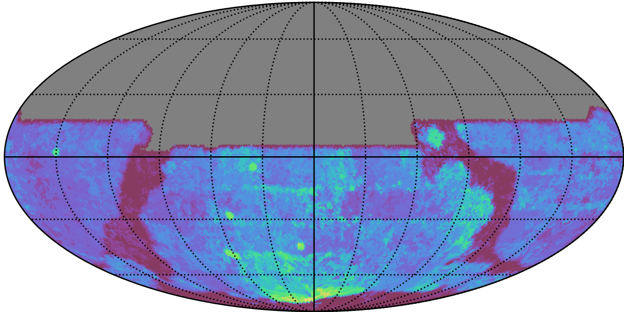
roll_uniform_eh_acc1.0_mjdp0_v3.4_10yrs All sky y band: Median Season Length
