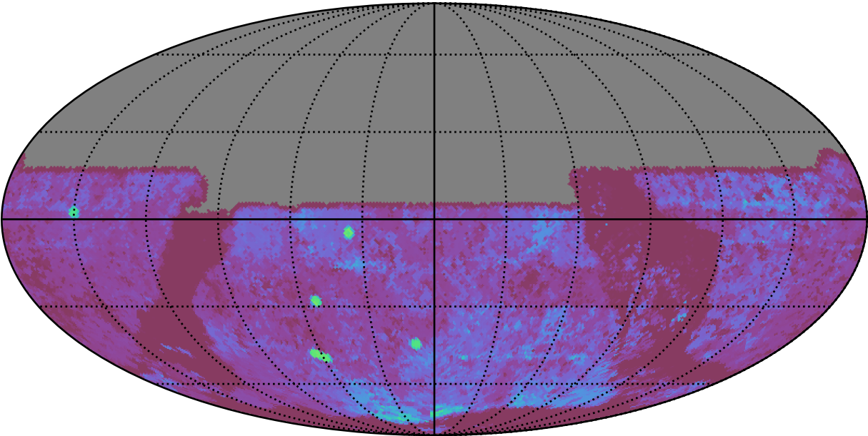
roll_uniform_eh_acc1.0_mjdp0_v3.4_10yrs All sky u band: Median Season Length
