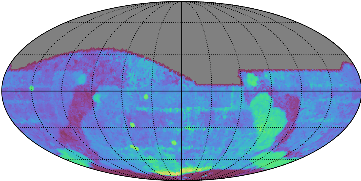
roll_uniform_eh_acc1.0_mjdp0_v3.4_10yrs All sky r band: Median Season Length
