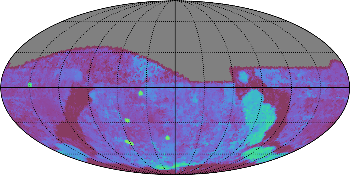
roll_uniform_eh_acc1.0_mjdp0_v3.4_10yrs All sky g band: Median Season Length
