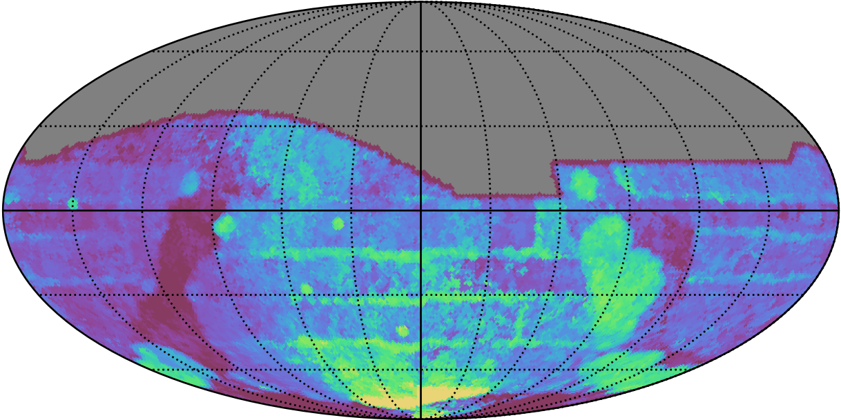
roll_uniform_eh_acc1.0_mjdp0_v3.4_10yrs All sky all bands: Median Season Length
