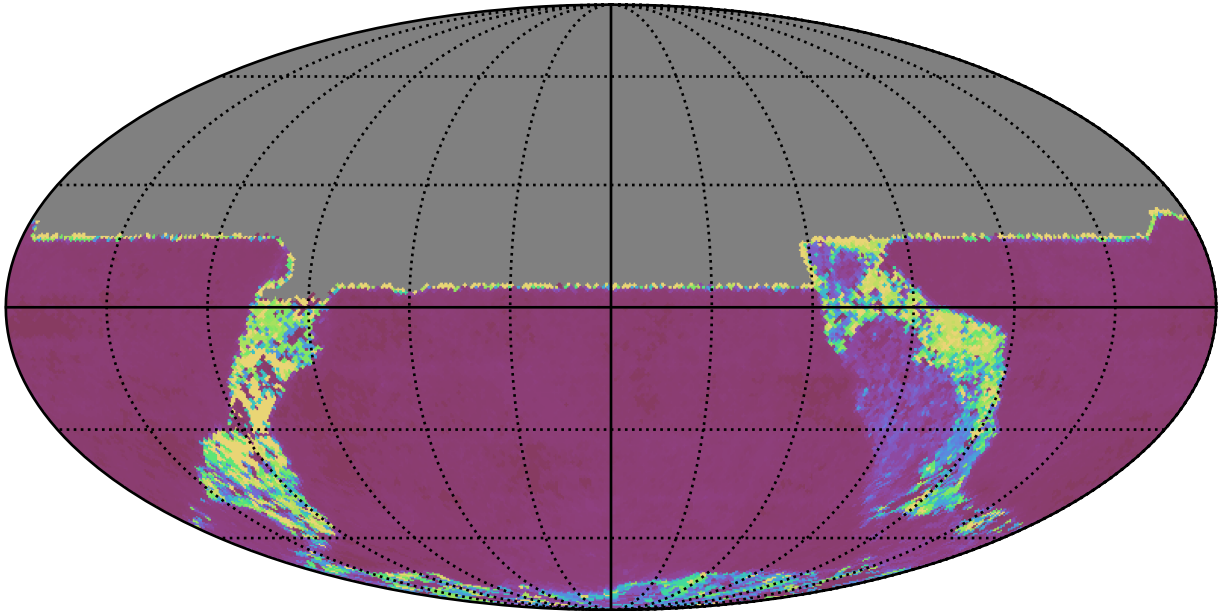
roll_uniform_eh_acc1.0_mjdp0_v3.4_10yrs All sky u band: Median Inter-Night Gap
