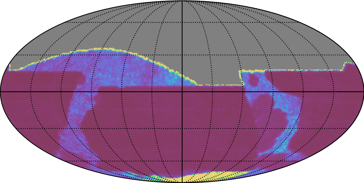
roll_uniform_eh_acc1.0_mjdp0_v3.4_10yrs All sky i band: Median Inter-Night Gap
