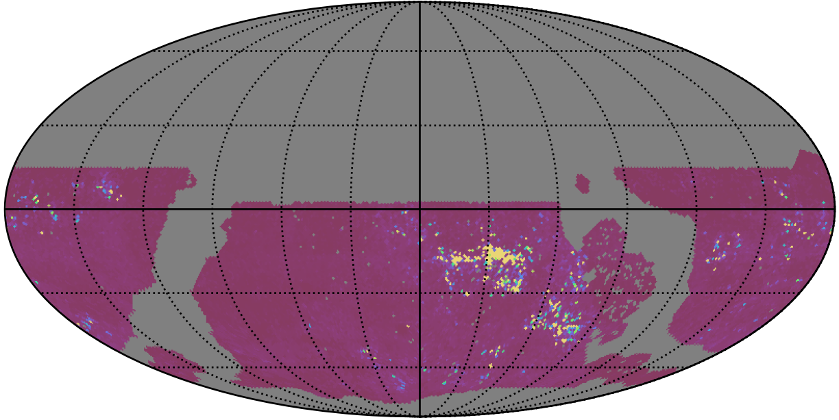
roll_uniform_eh_acc1.0_mjdp0_v3.4_10yrs WFD zy bands: 75th Percentile Intranight Timespan
