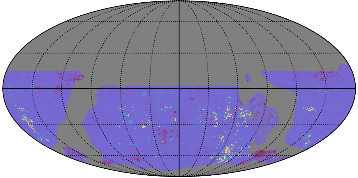
roll_uniform_eh_acc1.0_mjdp0_v3.4_10yrs WFD ug bands: 75th Percentile Intranight Timespan
