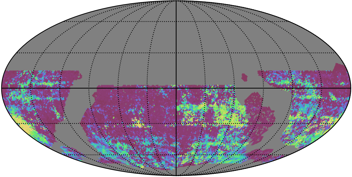
roll_uniform_eh_acc1.0_mjdp0_v3.4_10yrs WFD i band: 75th Percentile Intranight Timespan
