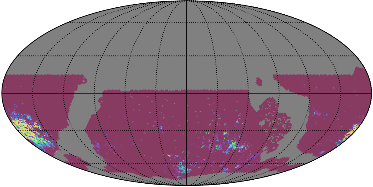
roll_uniform_eh_acc1.0_mjdp0_v3.4_10yrs WFD gr bands: 75th Percentile Intranight Timespan
