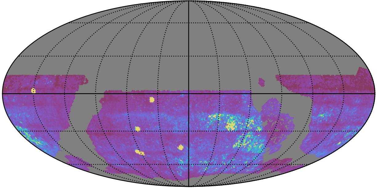
roll_uniform_eh_acc1.0_mjdp0_v3.4_10yrs WFD all bands: 75th Percentile Intranight Timespan
