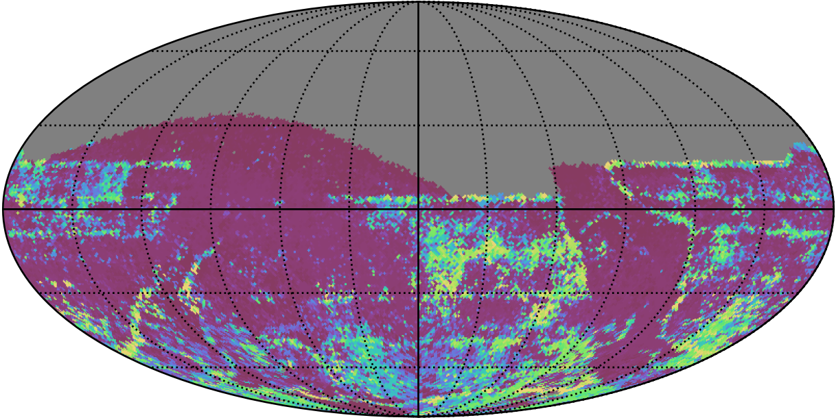
roll_uniform_eh_acc1.0_mjdp0_v3.4_10yrs All sky z band: 75th Percentile Intranight Timespan
