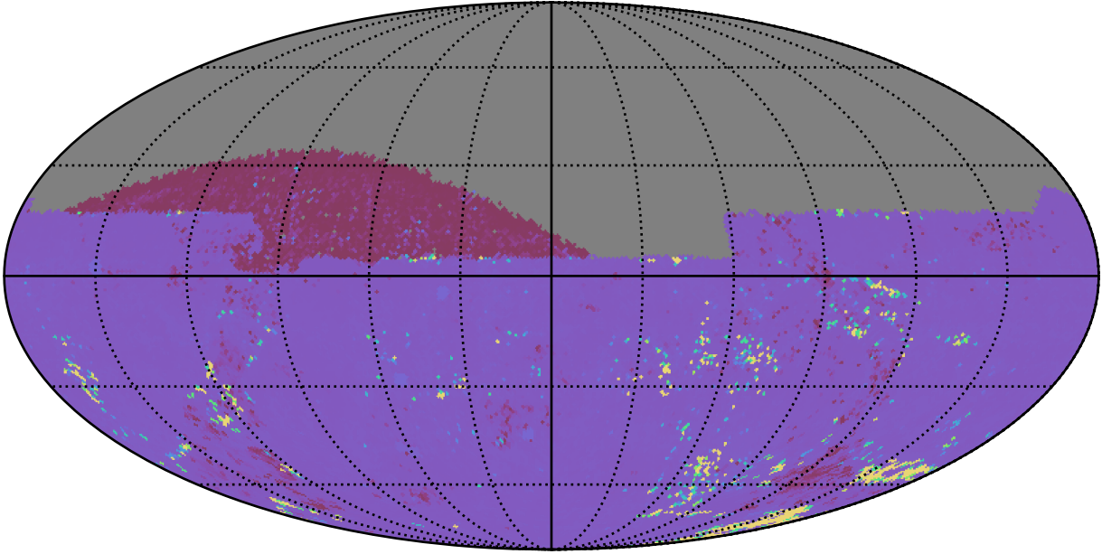
roll_uniform_eh_acc1.0_mjdp0_v3.4_10yrs All sky ug bands: 75th Percentile Intranight Timespan
