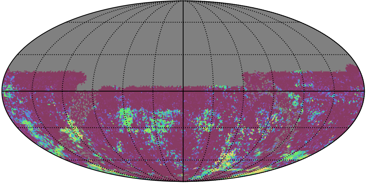
roll_uniform_eh_acc1.0_mjdp0_v3.4_10yrs All sky u band: 75th Percentile Intranight Timespan
