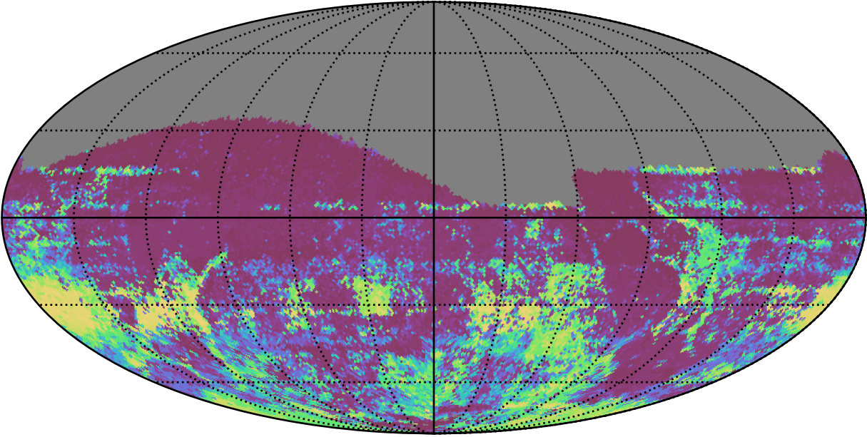
roll_uniform_eh_acc1.0_mjdp0_v3.4_10yrs All sky r band: 75th Percentile Intranight Timespan
