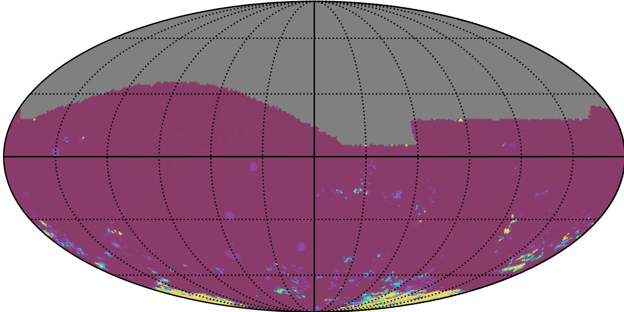
roll_uniform_eh_acc1.0_mjdp0_v3.4_10yrs All sky iz bands: 75th Percentile Intranight Timespan
