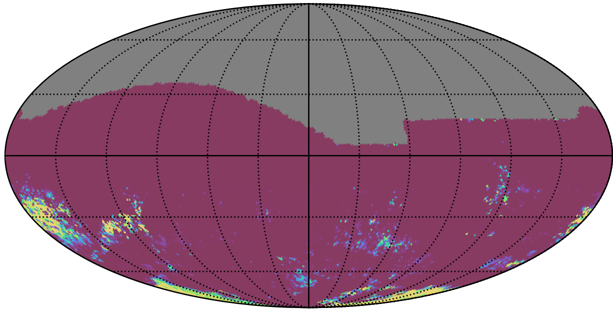
roll_uniform_eh_acc1.0_mjdp0_v3.4_10yrs All sky gr bands: 75th Percentile Intranight Timespan
