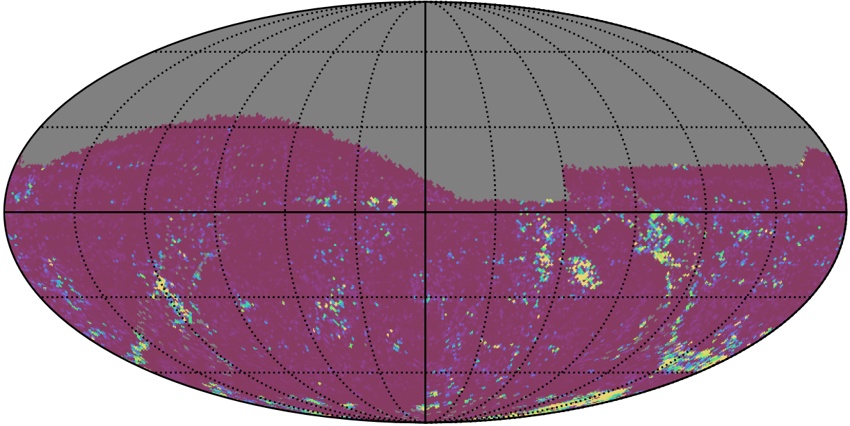
roll_uniform_eh_acc1.0_mjdp0_v3.4_10yrs All sky g band: 75th Percentile Intranight Timespan
