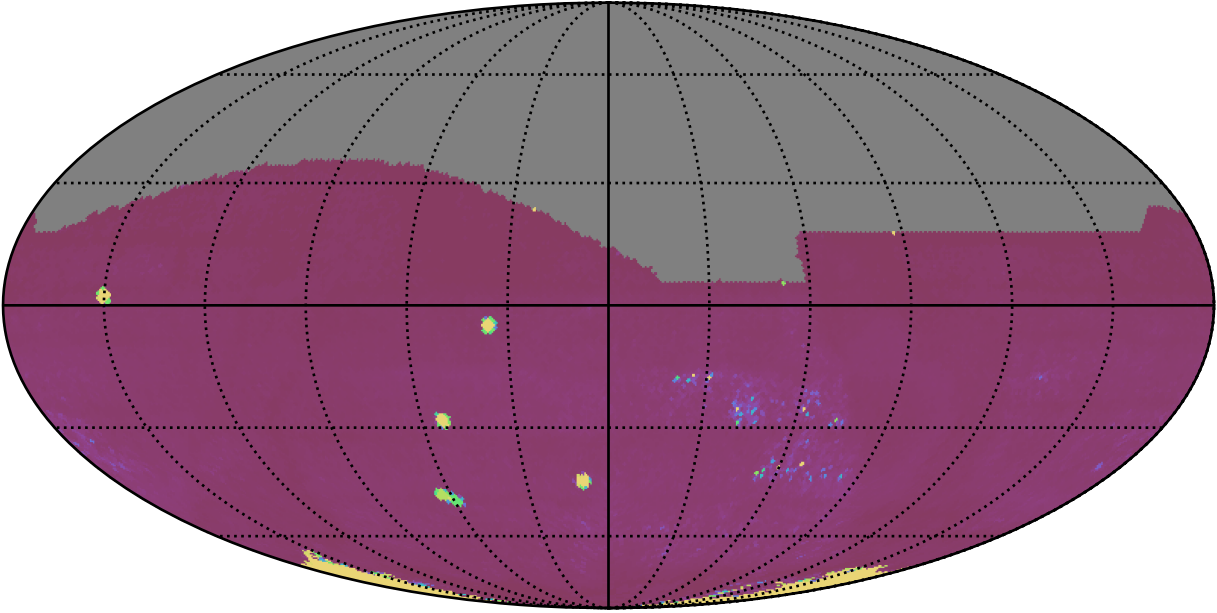
roll_uniform_eh_acc1.0_mjdp0_v3.4_10yrs All sky all bands: 75th Percentile Intranight Timespan
