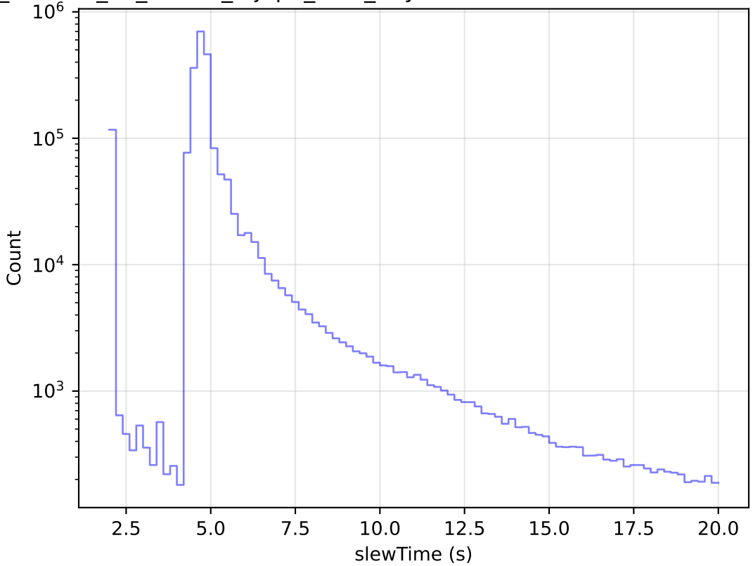
roll_uniform_eh_acc1.0_mjdp0_v3.4_10yrs All visits: Zoom Slew Time Histogram
