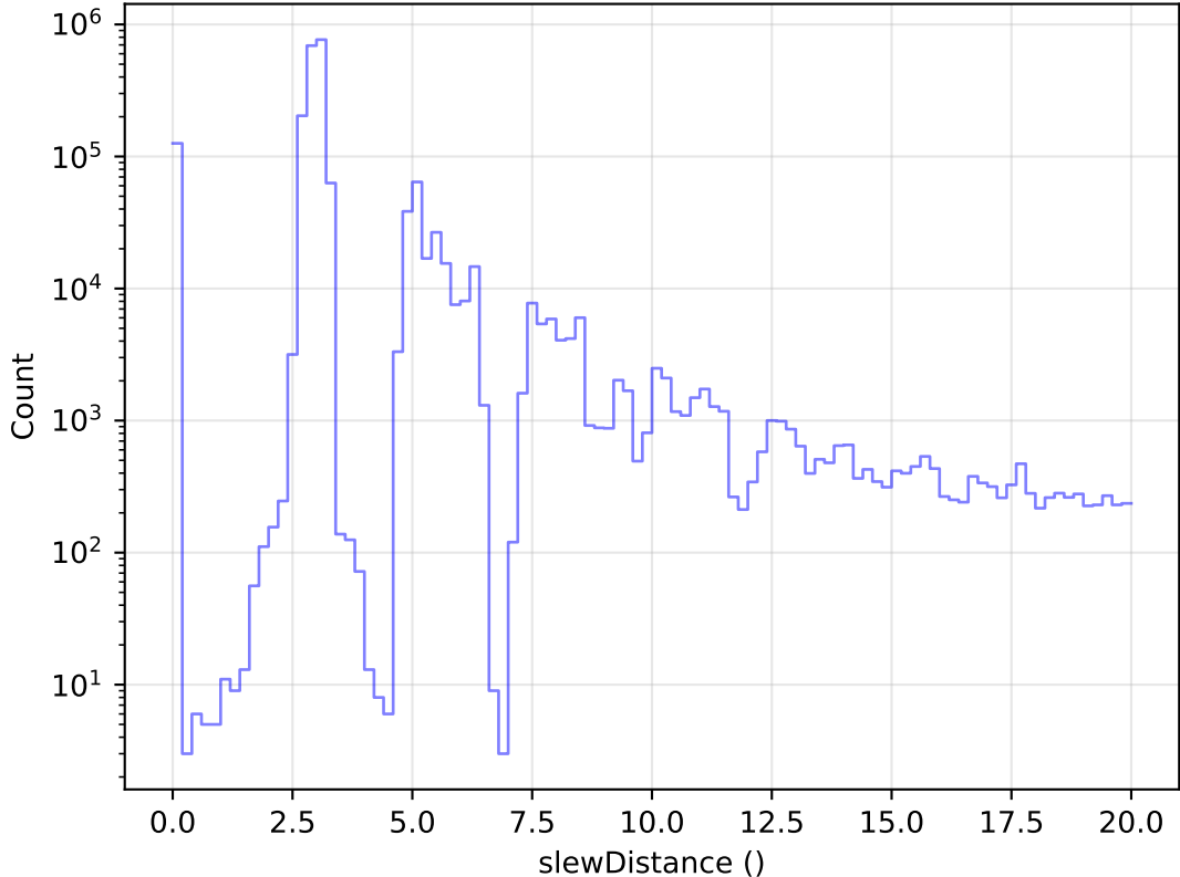
roll_uniform_eh_acc1.0_mjdp0_v3.4_10yrs All visits: Zoom Slew Distance Histogram
