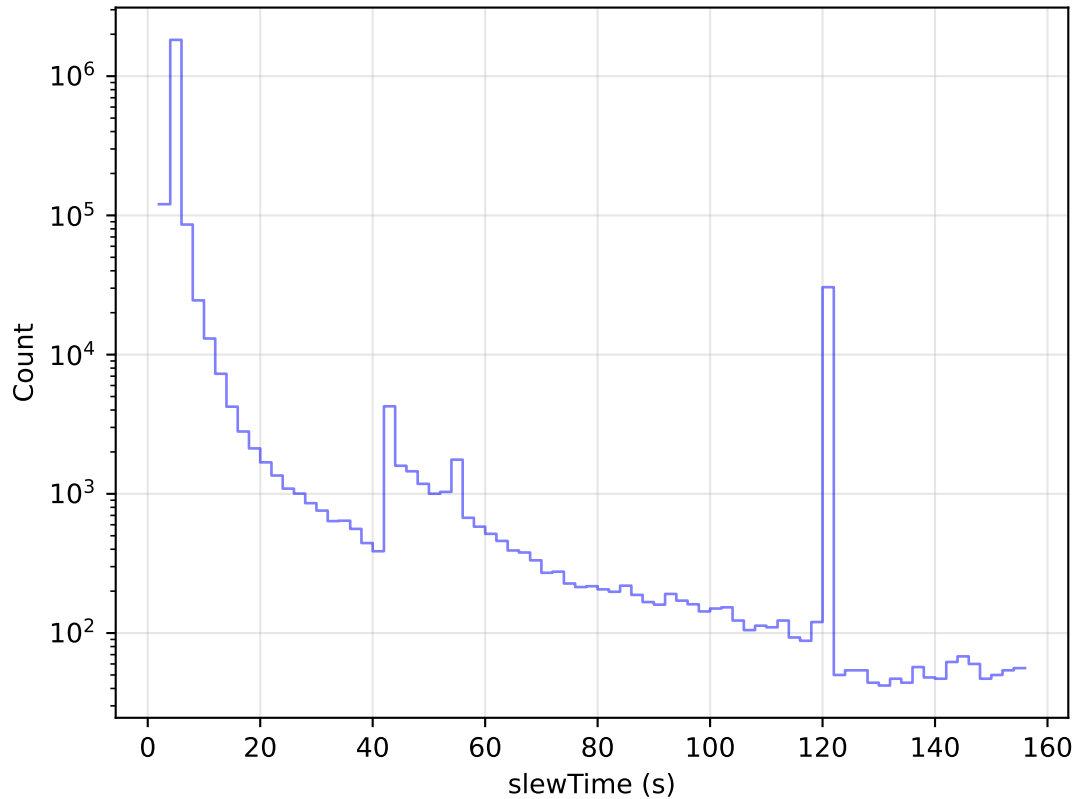
roll_uniform_eh_acc1.0_mjdp0_v3.4_10yrs All visits: Slew Time Histogram
