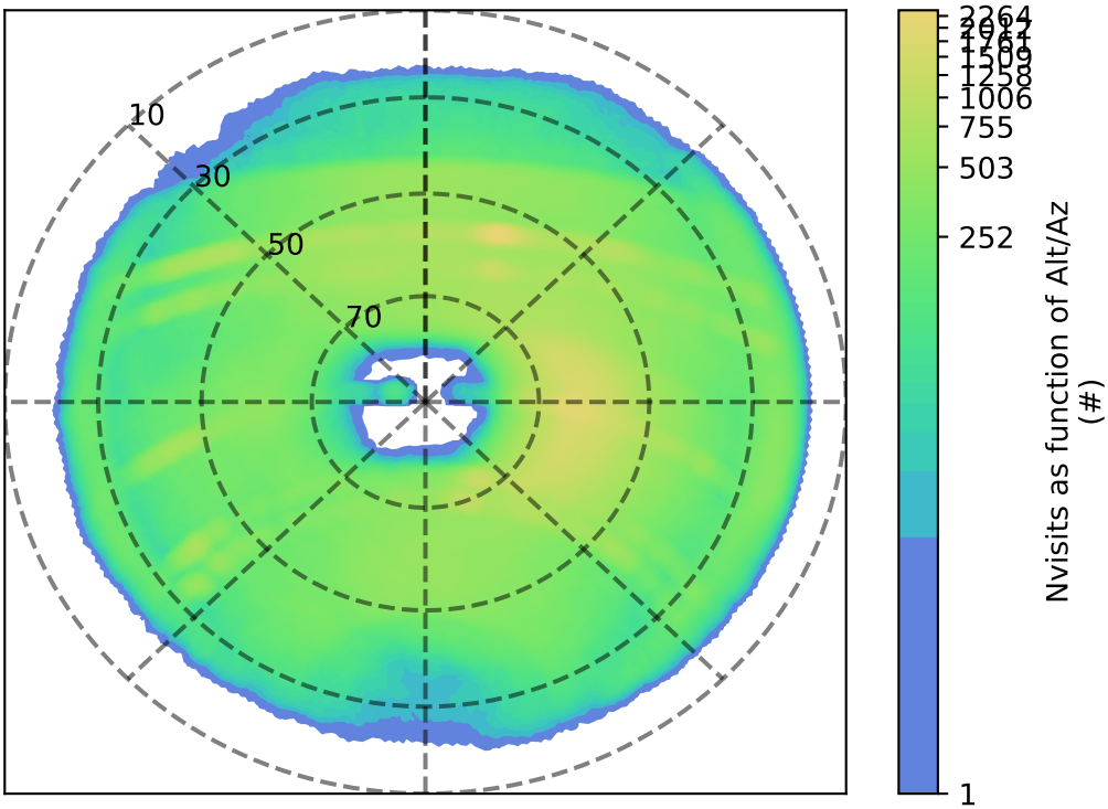
roll_uniform_eh_acc1.0_mjdp0_v3.4_10yrs z: Nvisits as function of Alt/Az
