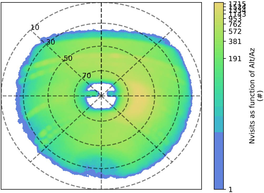
roll_uniform_eh_acc1.0_mjdp0_v3.4_10yrs y: Nvisits as function of Alt/Az
