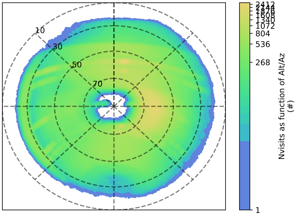
roll_uniform_eh_acc1.0_mjdp0_v3.4_10yrs r: Nvisits as function of Alt/Az
