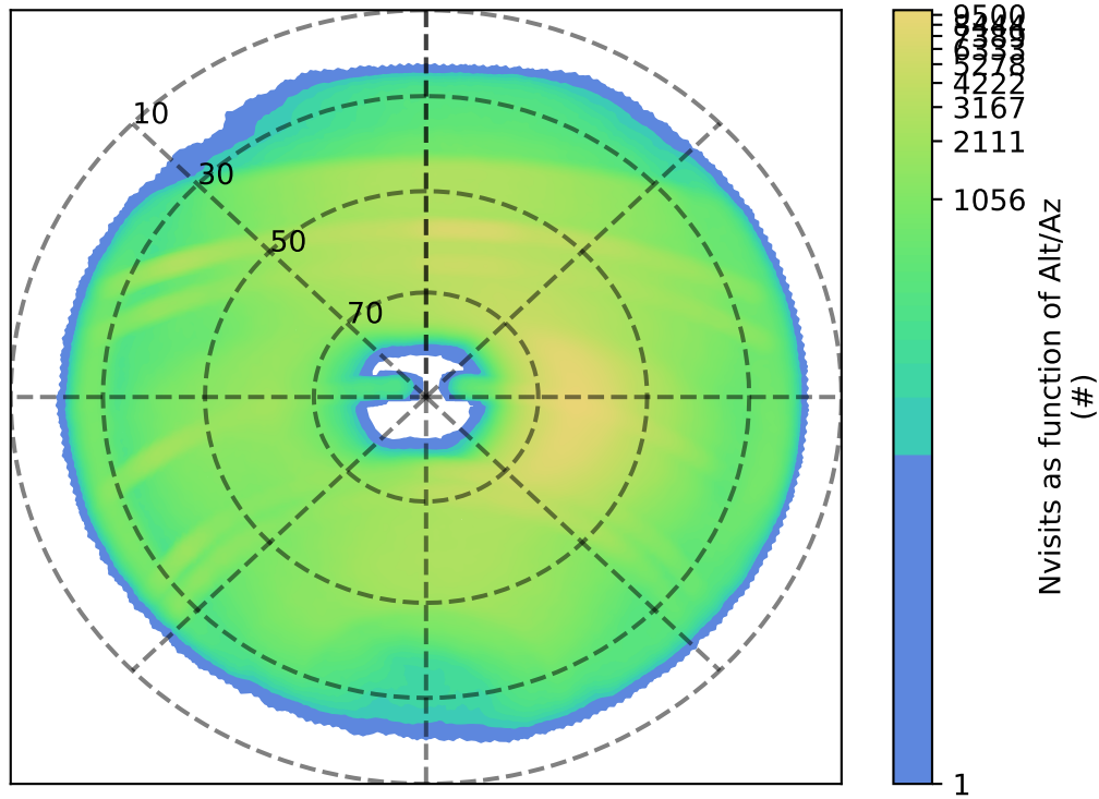
roll_uniform_eh_acc1.0_mjdp0_v3.4_10yrs : Nvisits as function of Alt/Az
