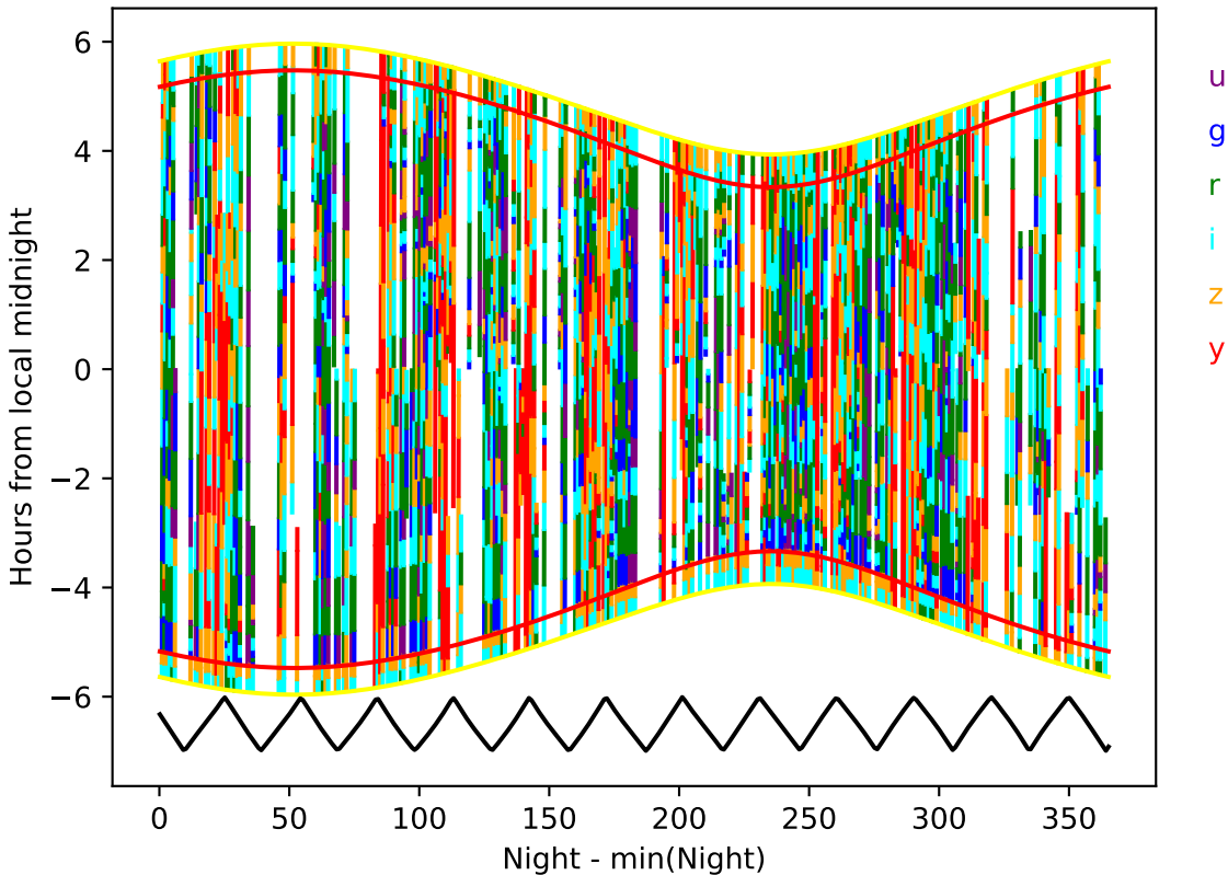
roll_uniform_eh_acc1.0_mjdp0_v3.4_10yrs year 7-8: Hourglass
