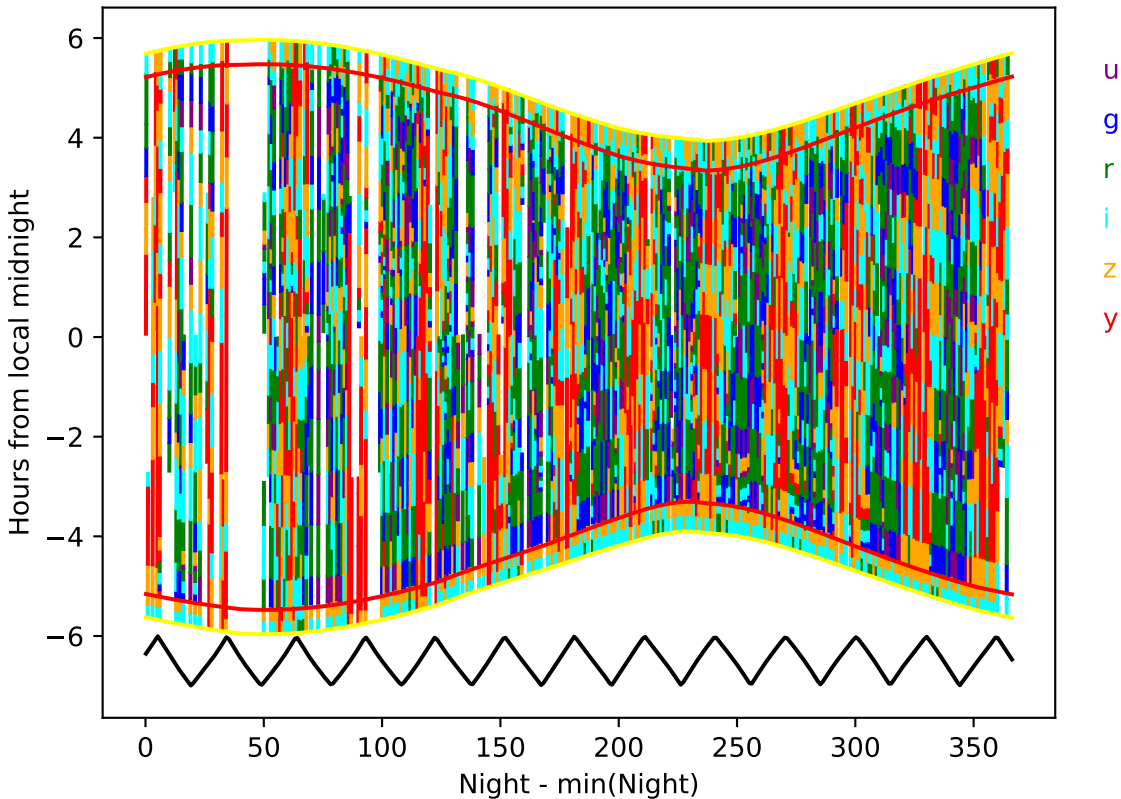
roll_uniform_eh_acc1.0_mjdp0_v3.4_10yrs year 6-7: Hourglass
