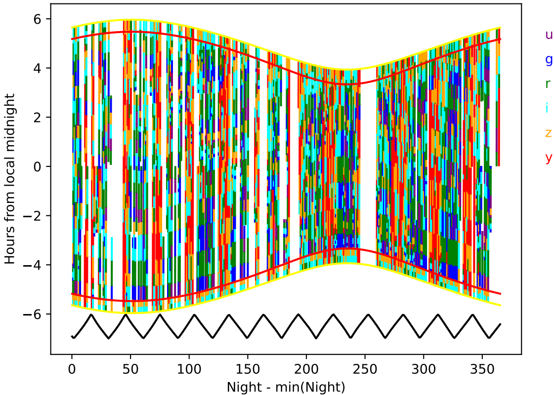
roll_uniform_eh_acc1.0_mjdp0_v3.4_10yrs year 5-6: Hourglass
