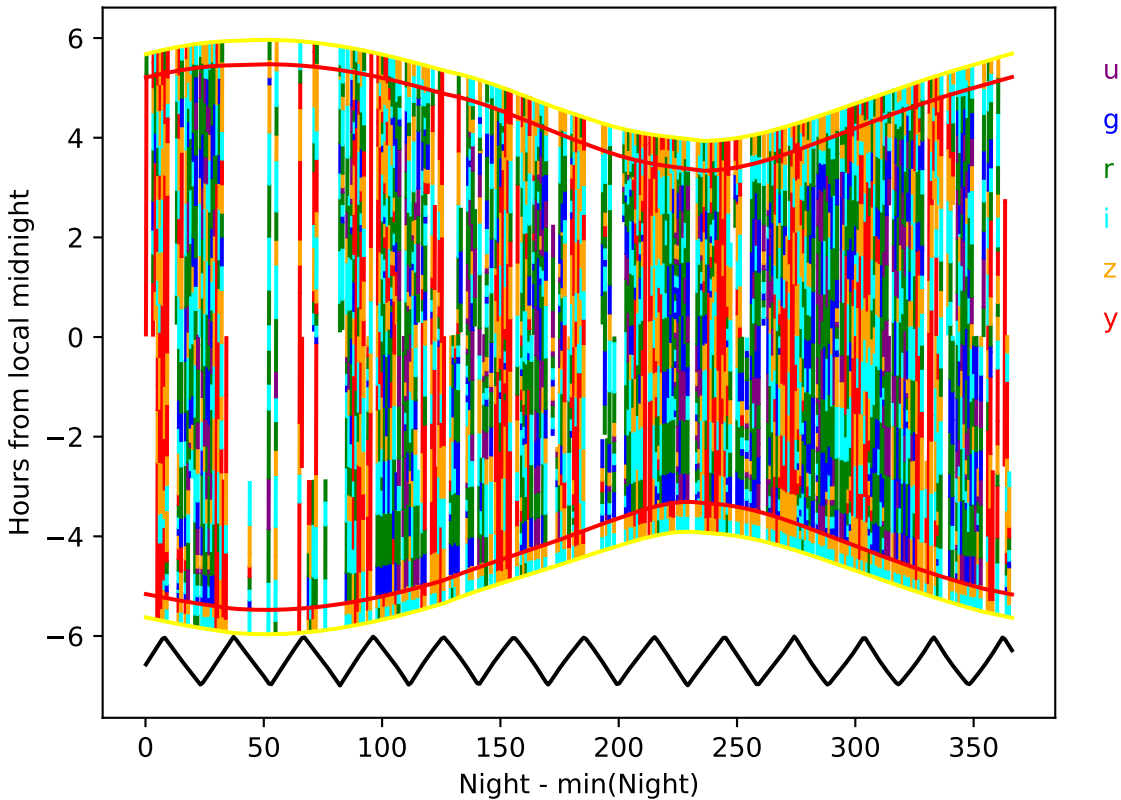
roll_uniform_eh_acc1.0_mjdp0_v3.4_10yrs year 3-4: Hourglass
