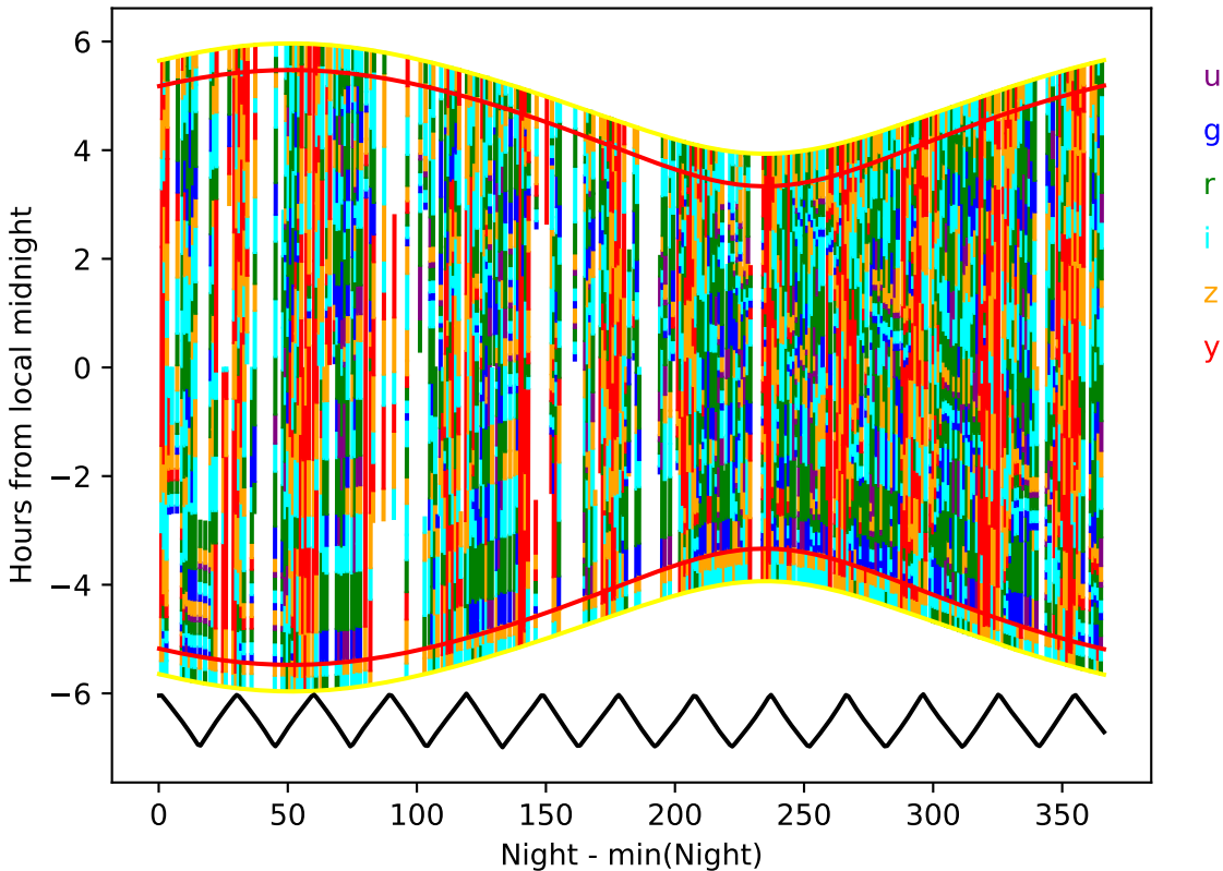
roll_uniform_eh_acc1.0_mjdp0_v3.4_10yrs year 1-2: Hourglass
