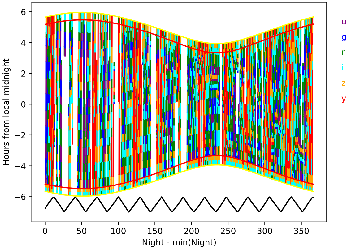
roll_uniform_eh_acc1.0_mjdp0_v3.4_10yrs year 0-1: Hourglass
