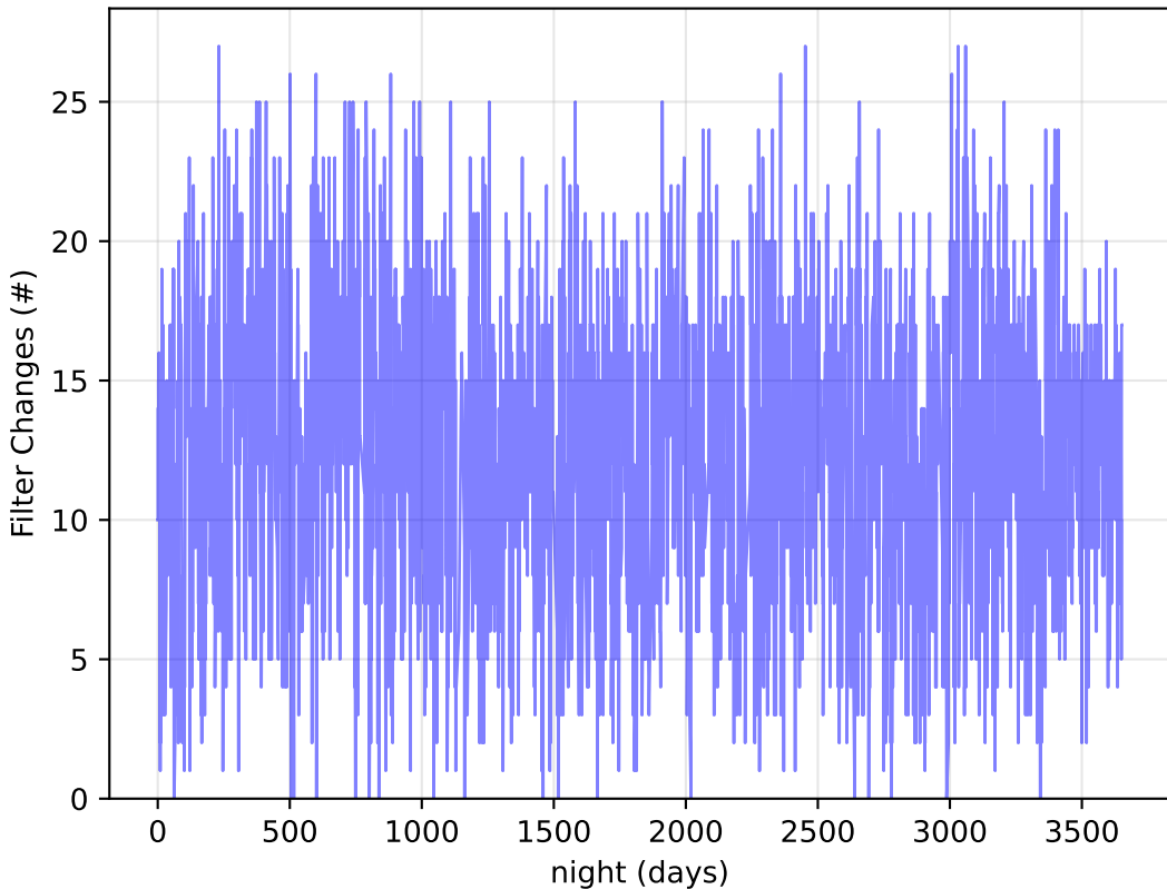
roll_uniform_eh_acc1.0_mjdp0_v3.4_10yrs : Filter Changes
