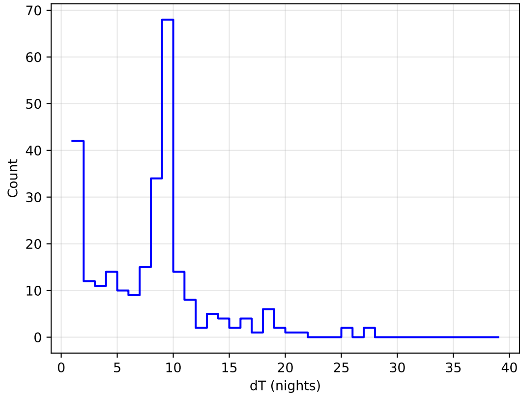
roll_uniform_eh_acc1.0_mjdp0_v3.4_10yrs all bands: DD:ELAISS1 Delta Nights Histogram
