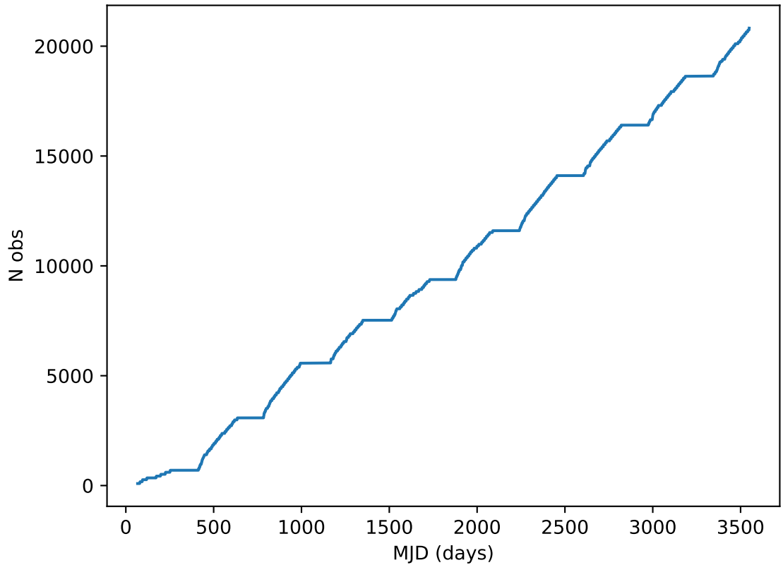
roll_uniform_eh_acc1.0_mjdp0_v3.4_10yrs all bands: DD:ELAISS1 Cumulative NVisits
