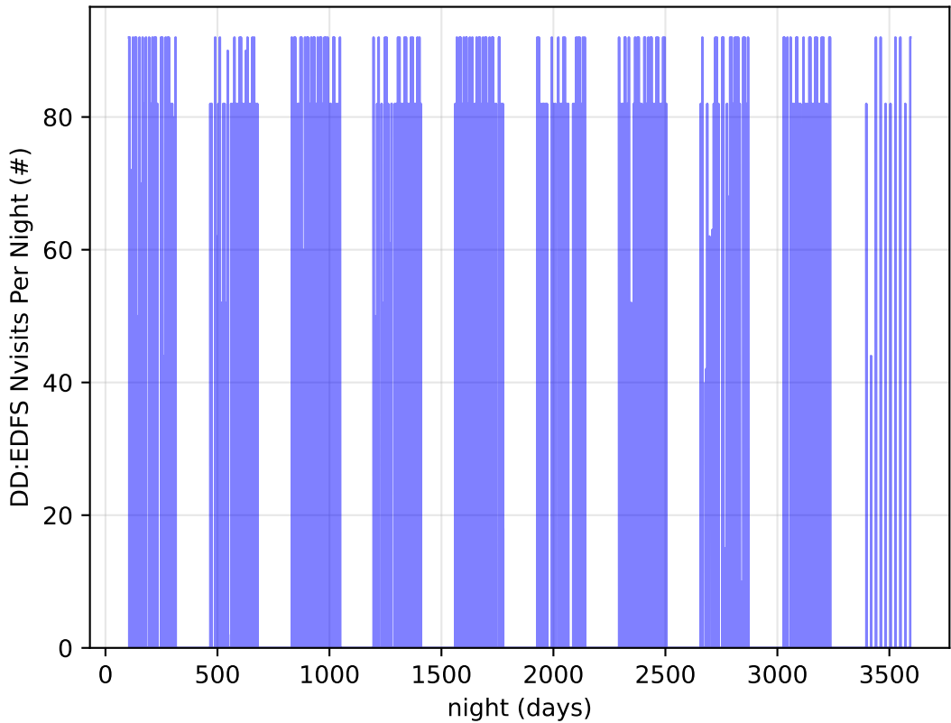
roll_uniform_eh_acc1.0_mjdp0_v3.4_10yrs all bands: DD:EDFS Nvisits Per Night
