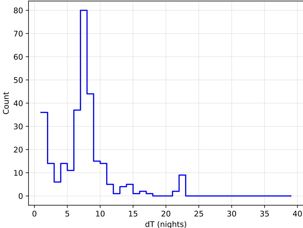
roll_uniform_eh_acc1.0_mjdp0_v3.4_10yrs all bands: DD:EDFS Delta Nights Histogram
